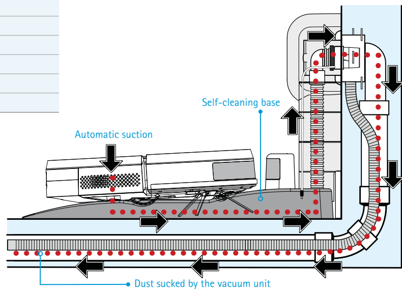
Diagram of the flow of dust from ROBÒ to the self-cleaning base
